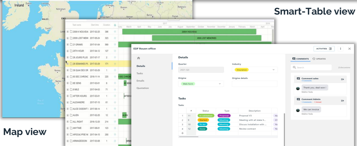
Gantt view
